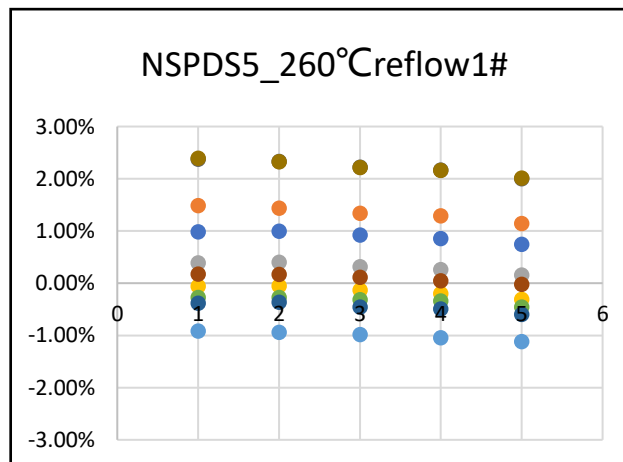
Fig 7.2 Test retest accuracy at reflux above standard temperature
