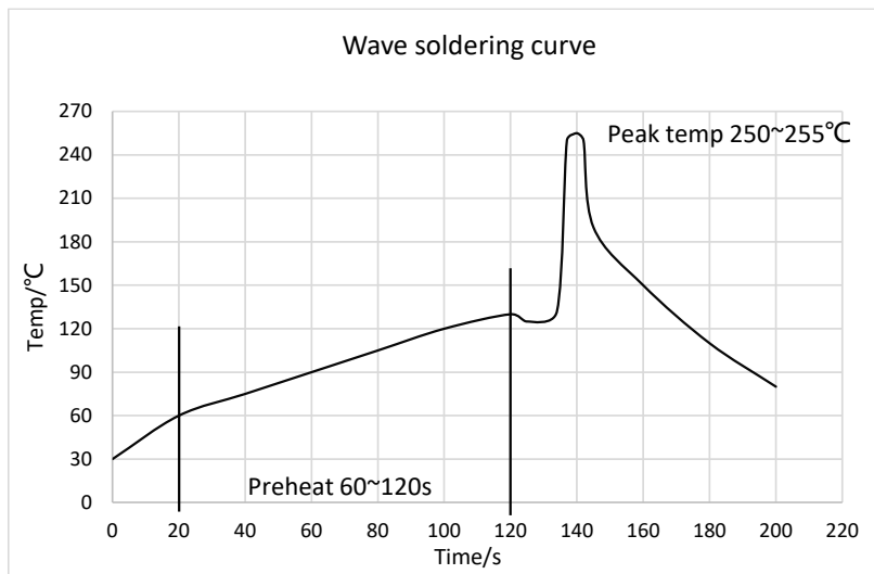
Fig 4.1 Wave Soldering Curve
