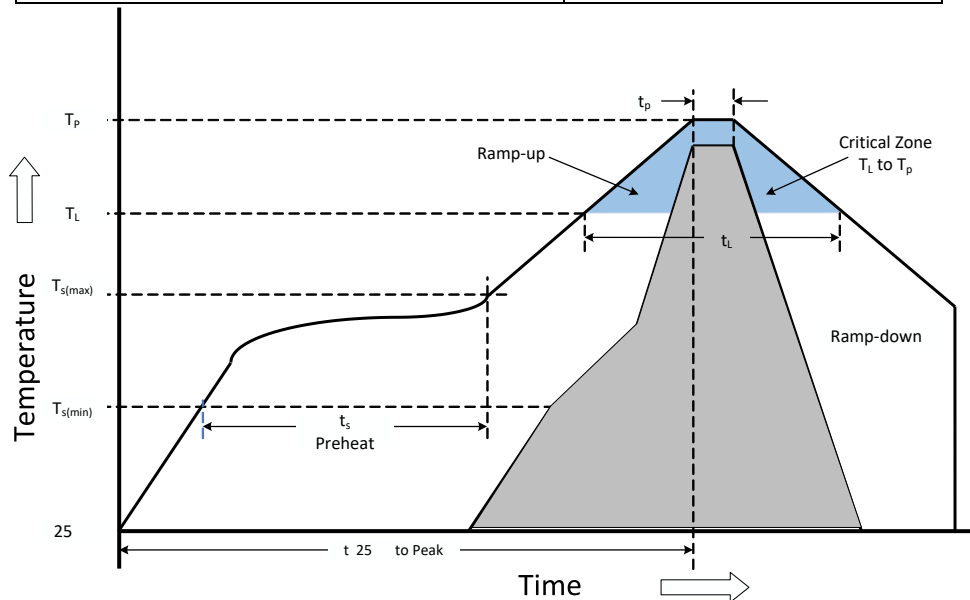
Fig 5.1 Reflow Soldering Curve
