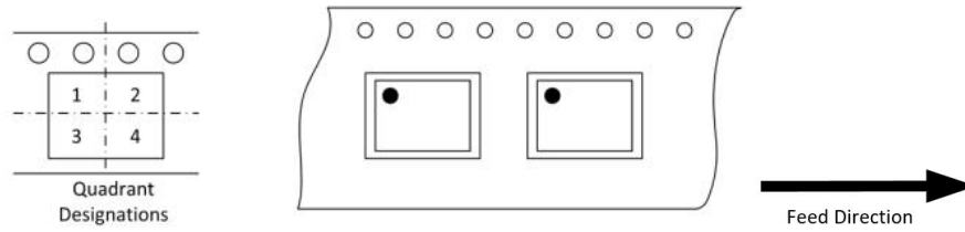
Figure 10.1 Tape and Reel Information of SOIC8
