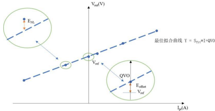
Figure 5.7 NSM2016 灵敏度及误差定义
