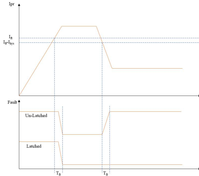
Figure 6.2 NSM2016 过流 Latch 表现
