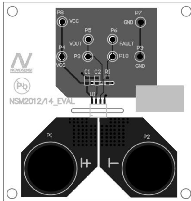
Figure 7.2 NSM2016 PCB Layout
