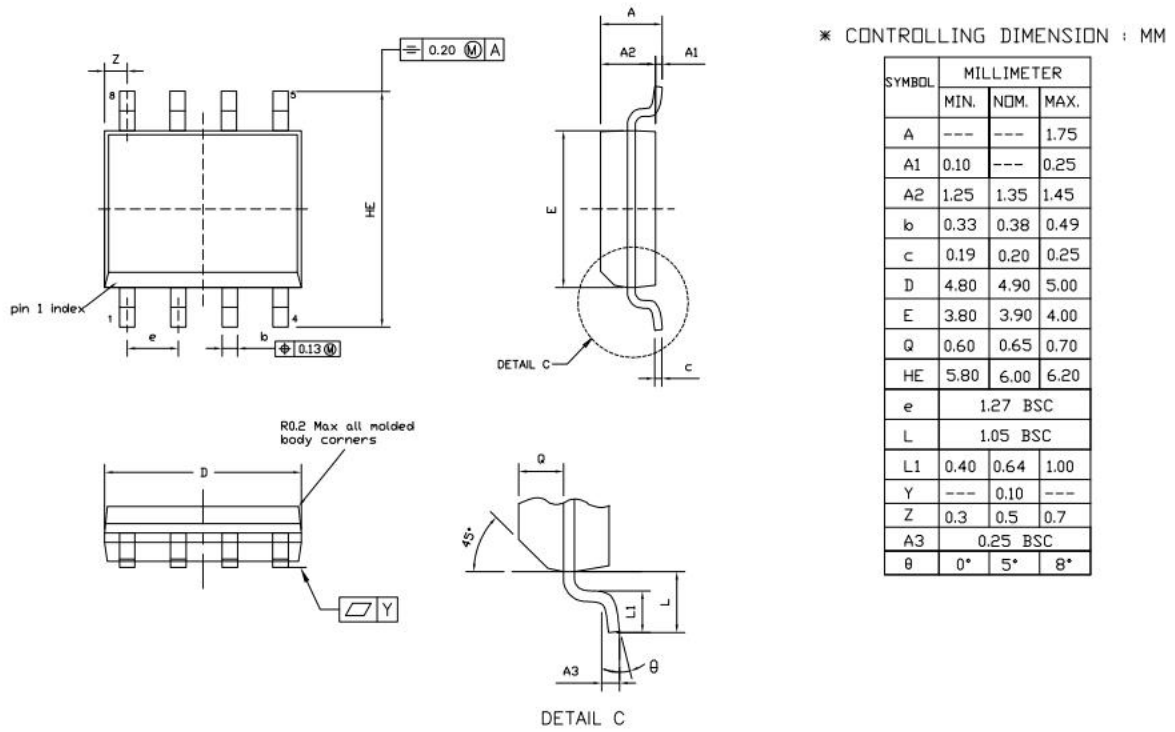
Figure 8.1 SOIC8 Package Shape and Dimension in millimeters
