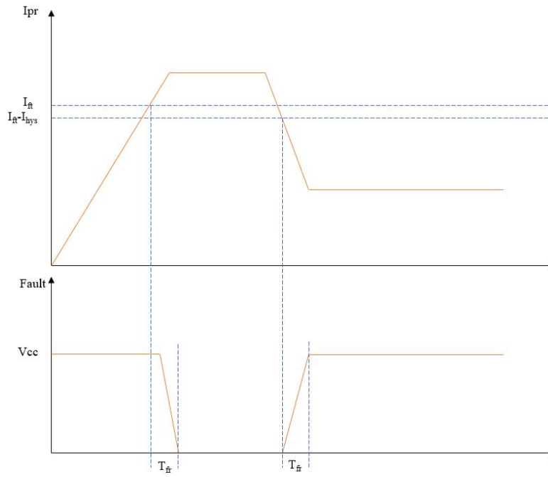
Figure 6.1 NSM2016 过流表现
