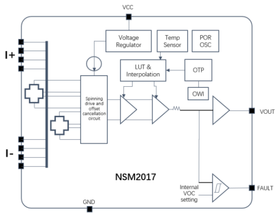
Figure 1. NSM2017 Block Diagram
