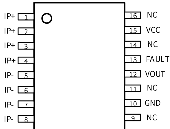
Figure 1.1 NSM2017 Package
