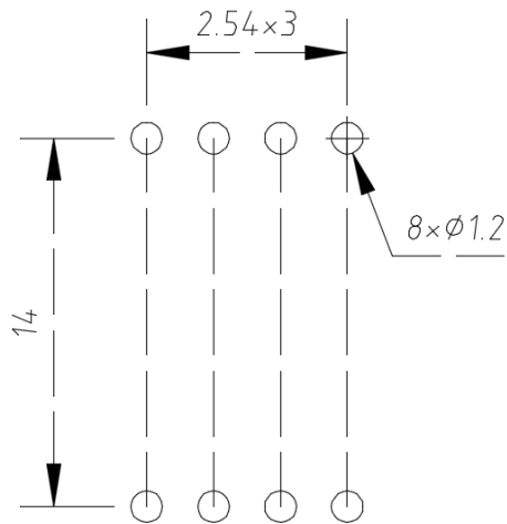
Figure 8.2 Footprint mm
