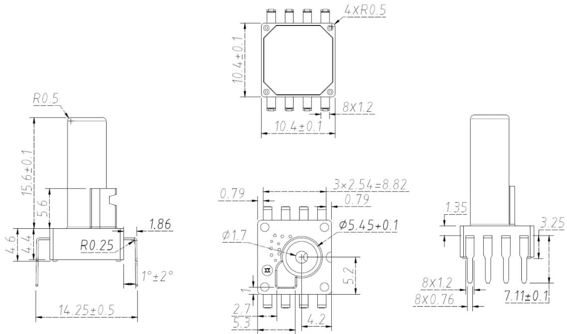
Figure 8.1 Package Outline mm
