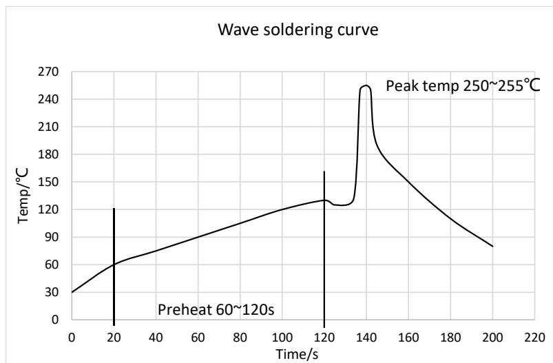
Figure 11.1 Wave Soldering Curve
