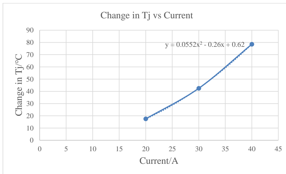
Figure 6.4 NSM2015 Estimation function of junction temperature at different currents (PCB is in worst case)
